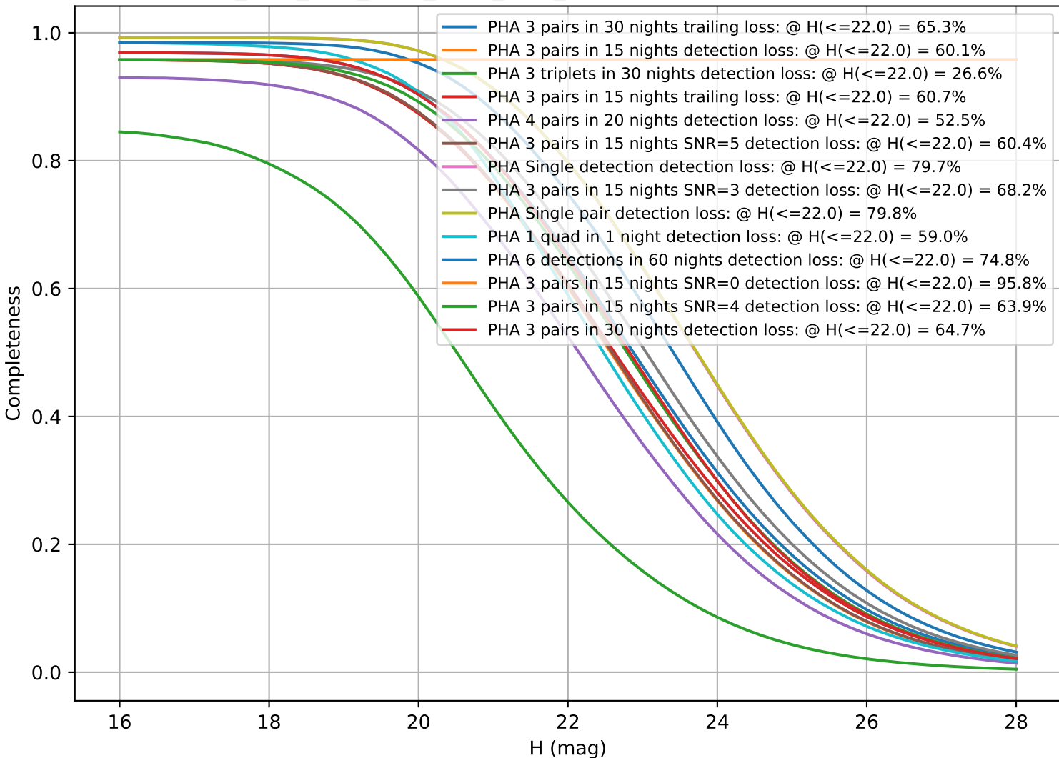
ddf_acor_sf20_lsf30_lsr10_v3.4_10yrs: CumulativeCompleteness
