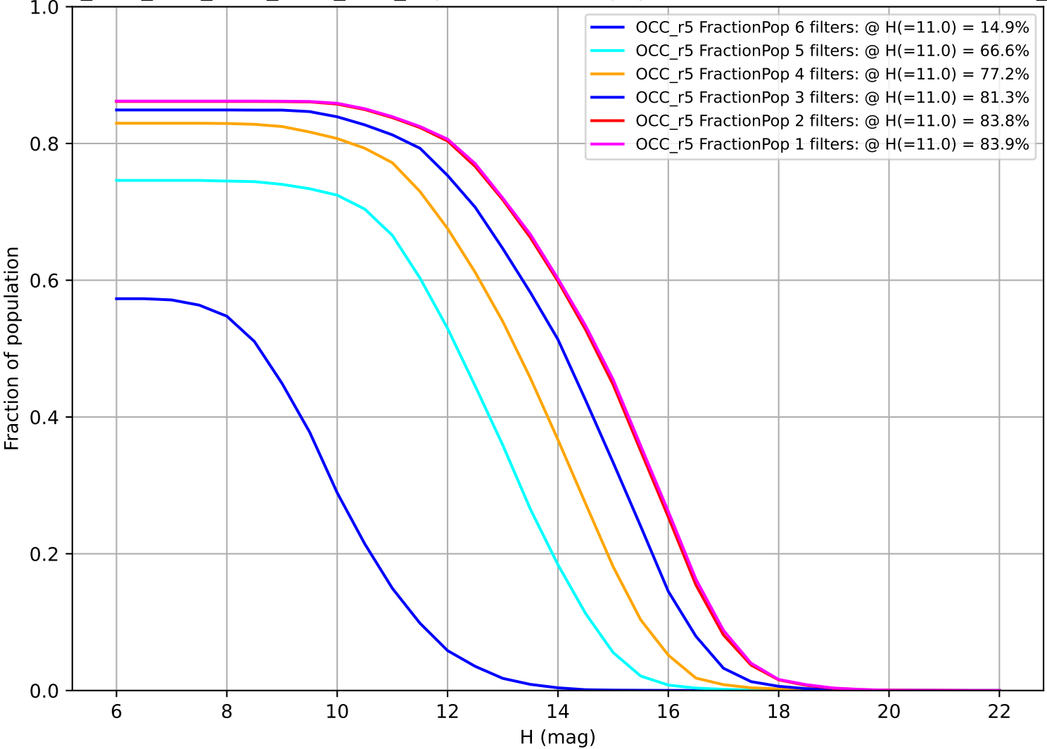
ddf_acor_sf20_lsf30_lsr10_v3.4_10yrs: Fraction of population with colors in X filters OCC_r5
