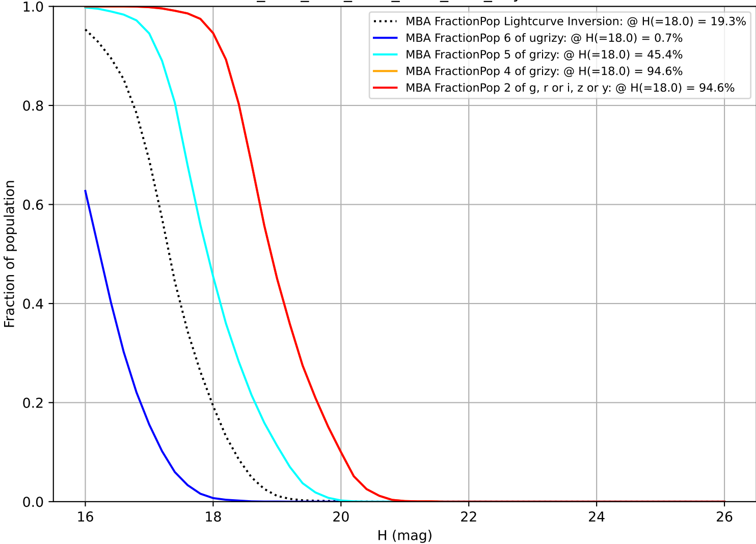
ddf_acor_sf20_lsf30_lsr10_v3.4_10yrs MBA
