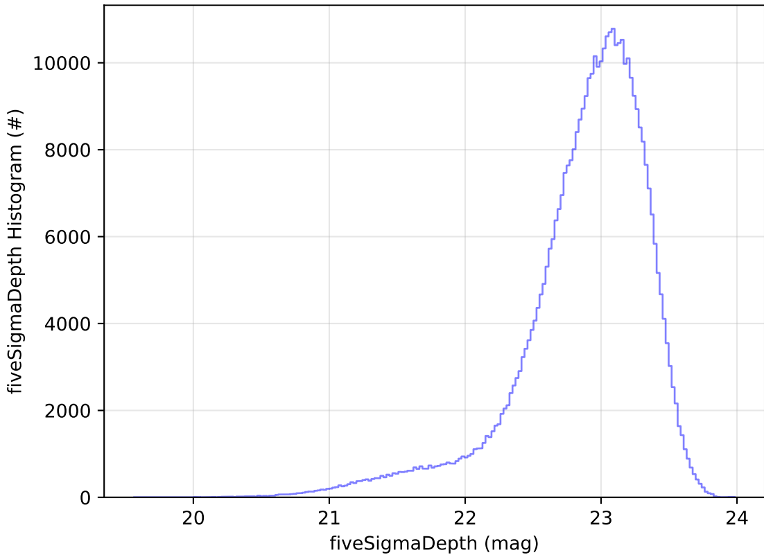
ddf_acor_sf20_lsf30_lsr10_v3.4_10yrs z: fiveSigmaDepth Histogram
