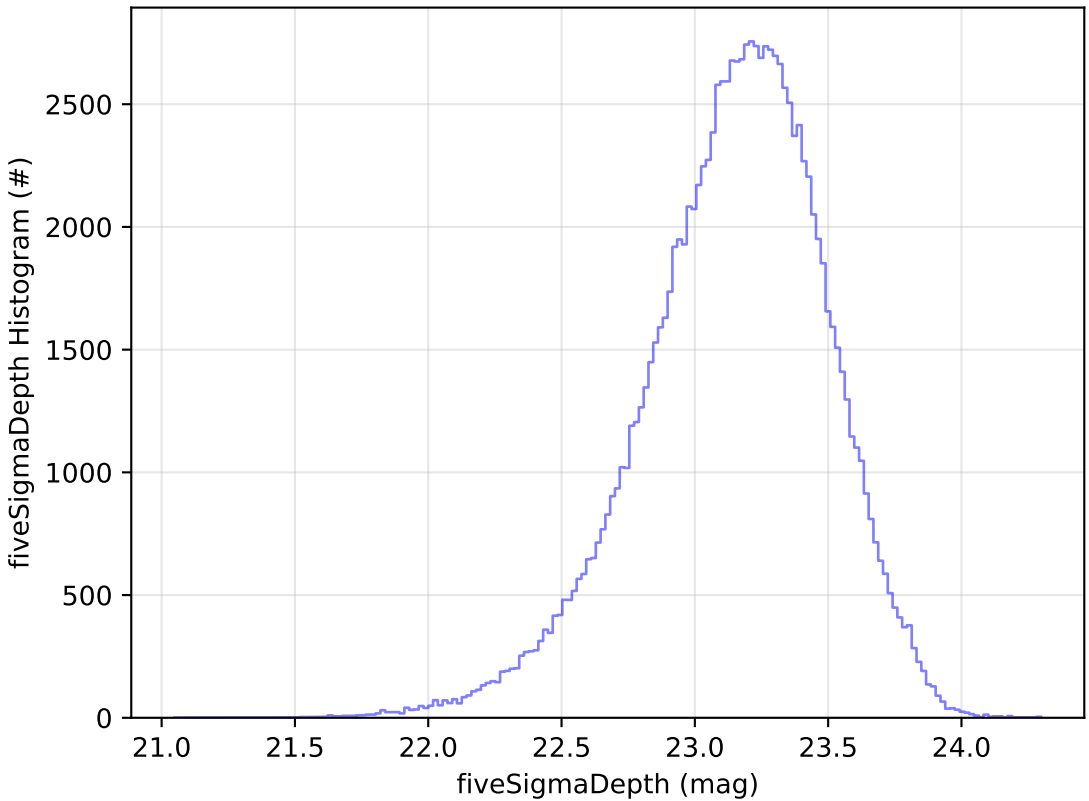
ddf_acor_sf20_lsf30_lsr10_v3.4_10yrs u: fiveSigmaDepth Histogram
