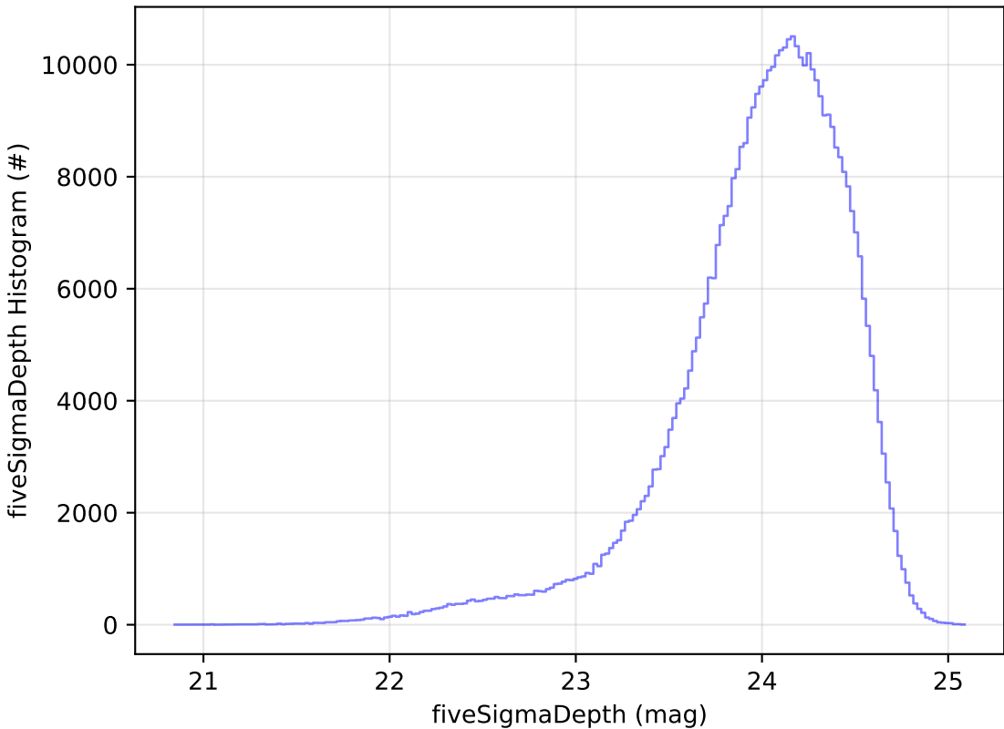
ddf_acor_sf20_lsf30_lsr10_v3.4_10yrs r: fiveSigmaDepth Histogram
