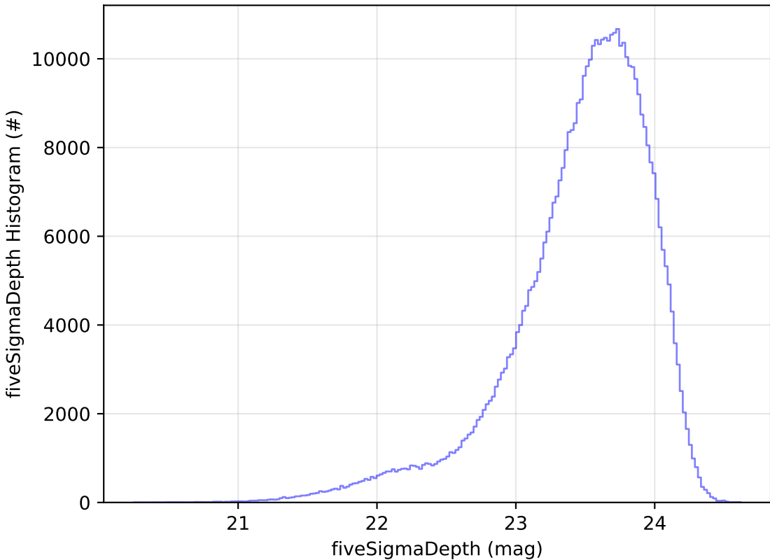
ddf_acor_sf20_lsf30_lsr10_v3.4_10yrs i: fiveSigmaDepth Histogram
