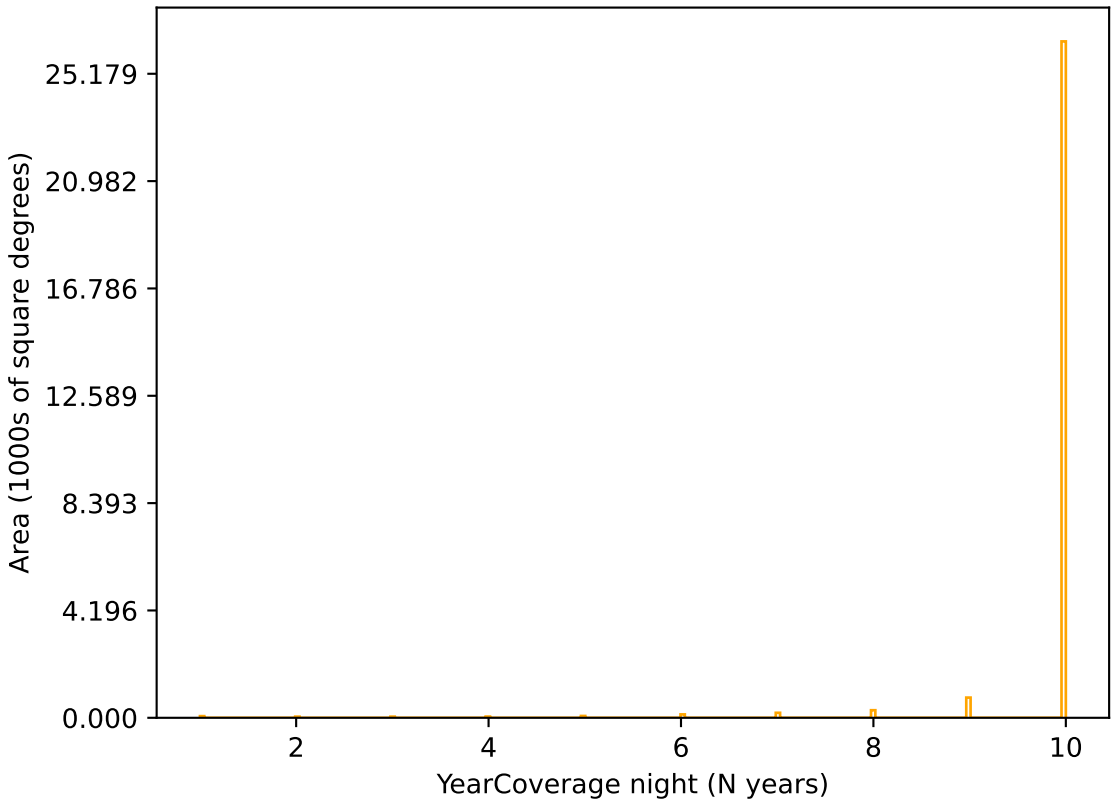
ddf_acor_sf20_lsf30_lsr10_v3.4_10yrs r band: YearCoverage night
