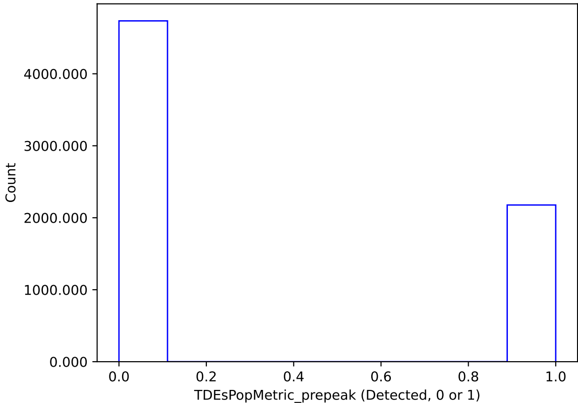
ddf_acor_sf20_lsf30_lsr10_v3.4_10yrs : TDEsPopMetric_prepeak
