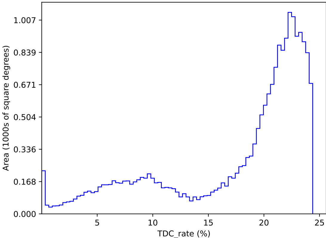
ddf_acor_sf20_lsf30_lsr10_v3.4_10yrs : TDC_rate
