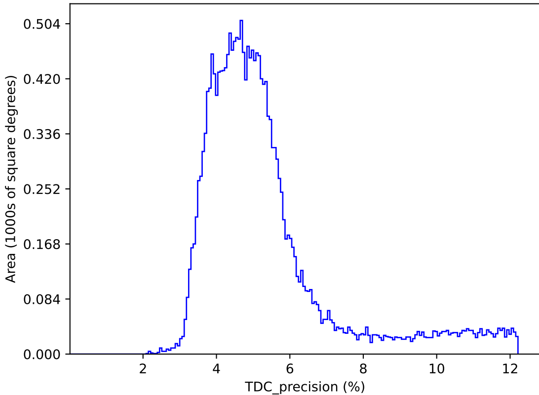
ddf_acor_sf20_lsf30_lsr10_v3.4_10yrs : TDC_precision
