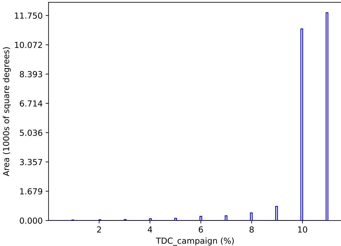
ddf_acor_sf20_lsf30_lsr10_v3.4_10yrs : TDC_campaign
