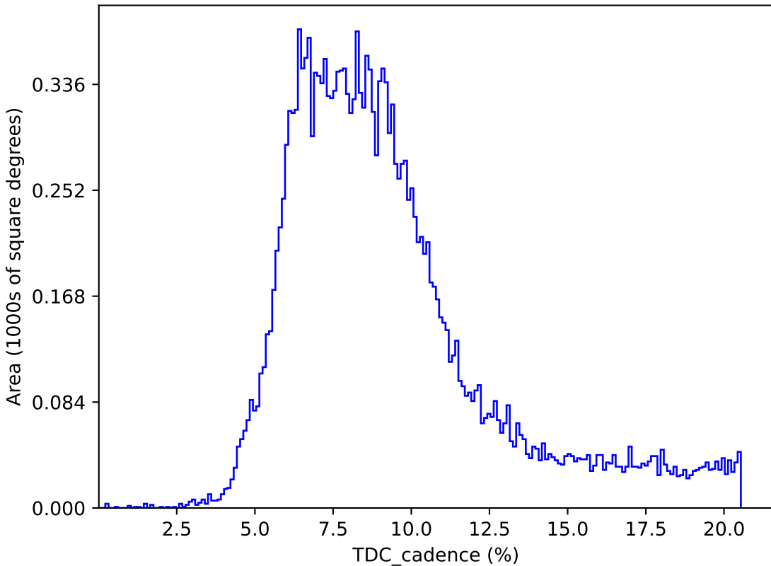
ddf_acor_sf20_ls30_lsr10_v3.4_10yrs : TDC_cadence
