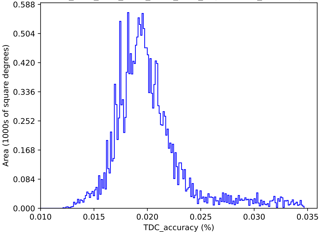
ddf_acor_sf20_lsf30_lsr10_v3.4_10yrs : TDC_accuracy
