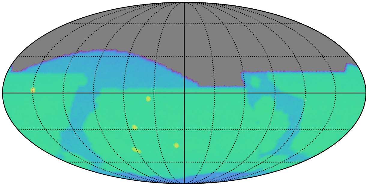
ddf_acor_sf20_lsf30_lsr10_v3.4_10yrs i: SurfaceBrightLimit
