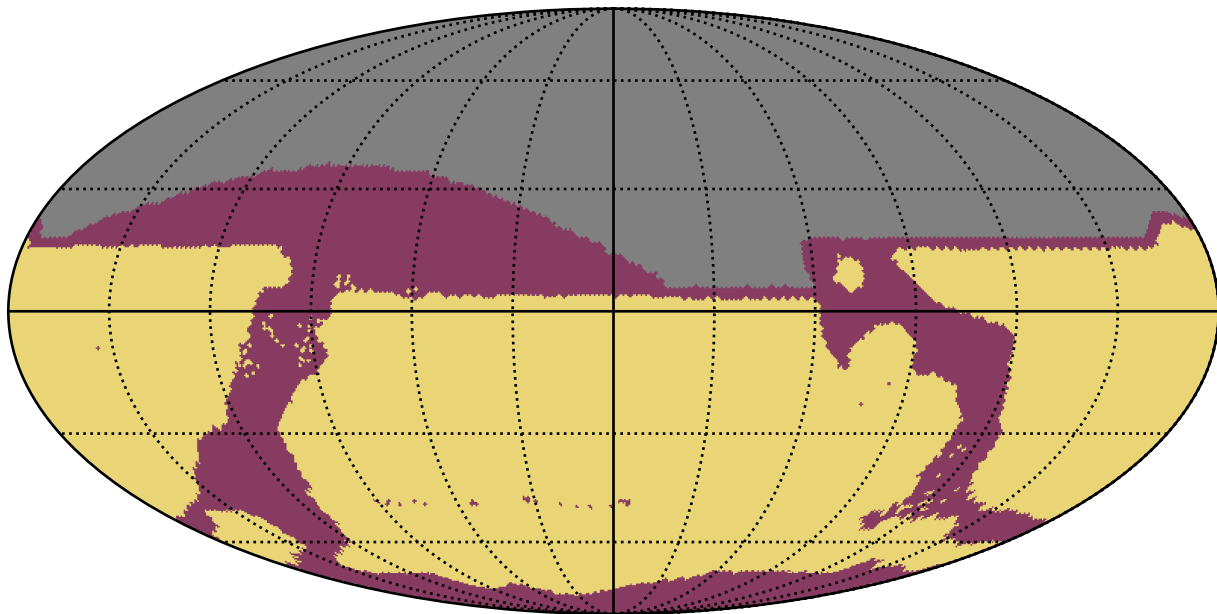
ddf_acor_sf20_lsf30_lsr10_v3.4_10yrs : RapidRevisits
