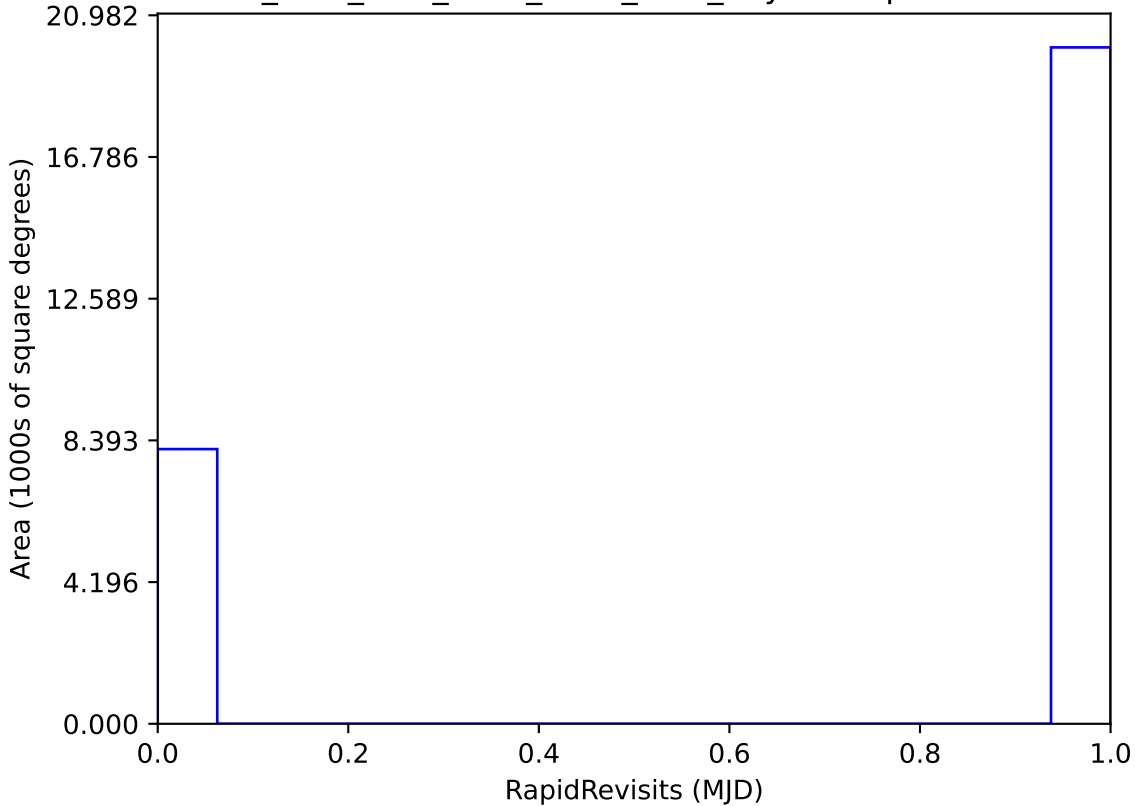
ddf_acor_sf20_lsf30_lsr10_v3.4_10yrs : RapidRevisits
