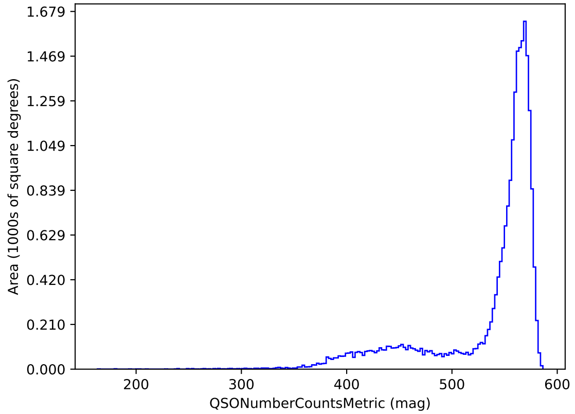
ddf_acor_sf20_lsf30_lsr10_v3.4_10yrs y band and non-DD: QSONumberCountsMetric
