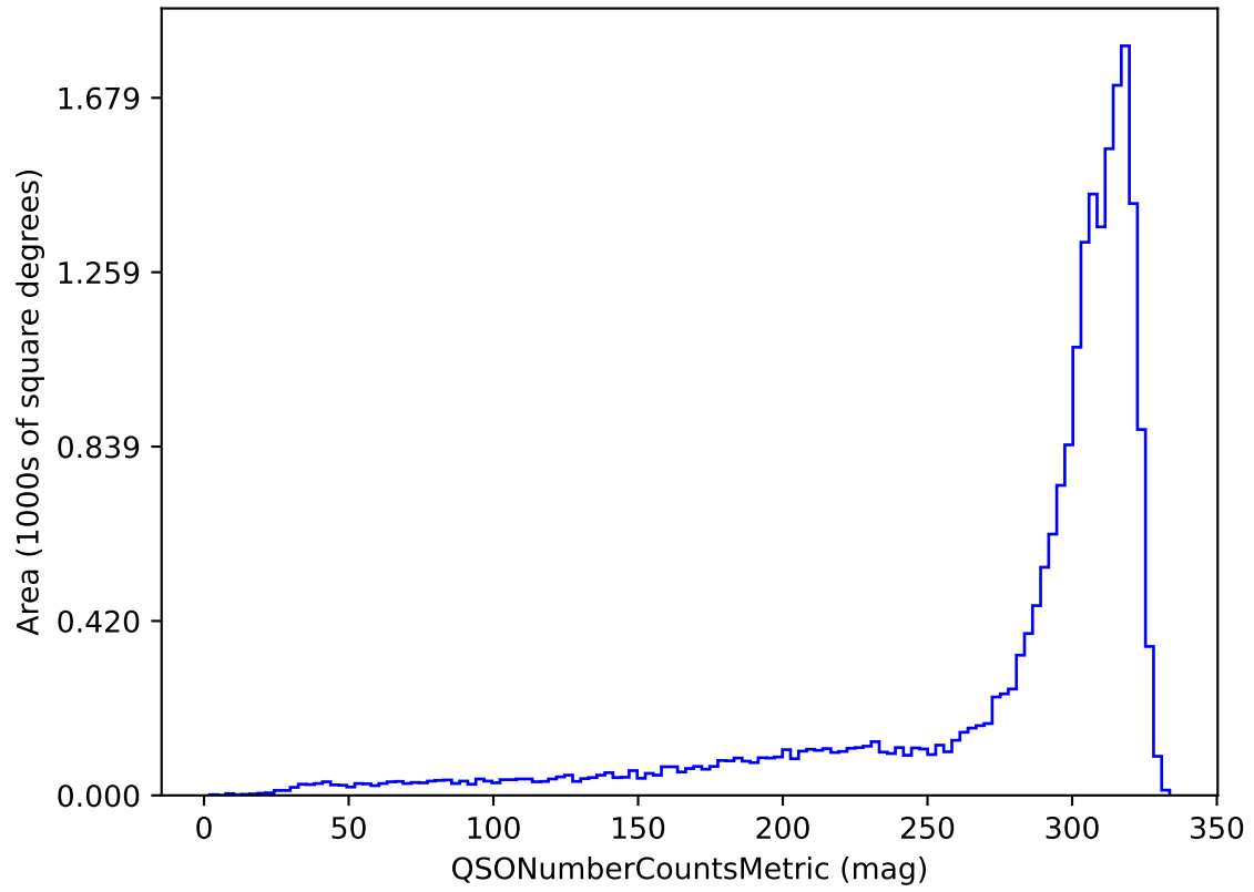
ddf_acor_sf20_lsf30_lsr10_v3.4_10yrs u band and non-DD: QSONumberCountsMetric
