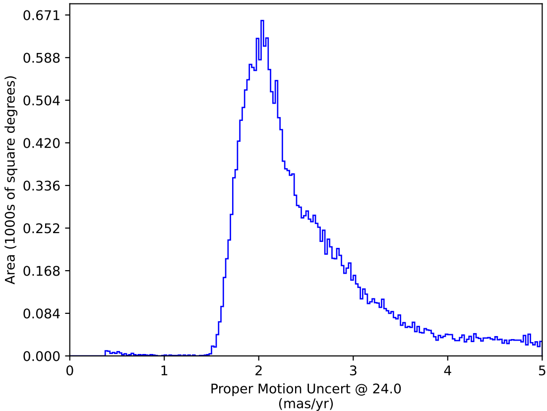
ddf_acor_sf20_lsf30_lsr10_v3.4_10yrs : Proper Motion Uncert @ 24.0
