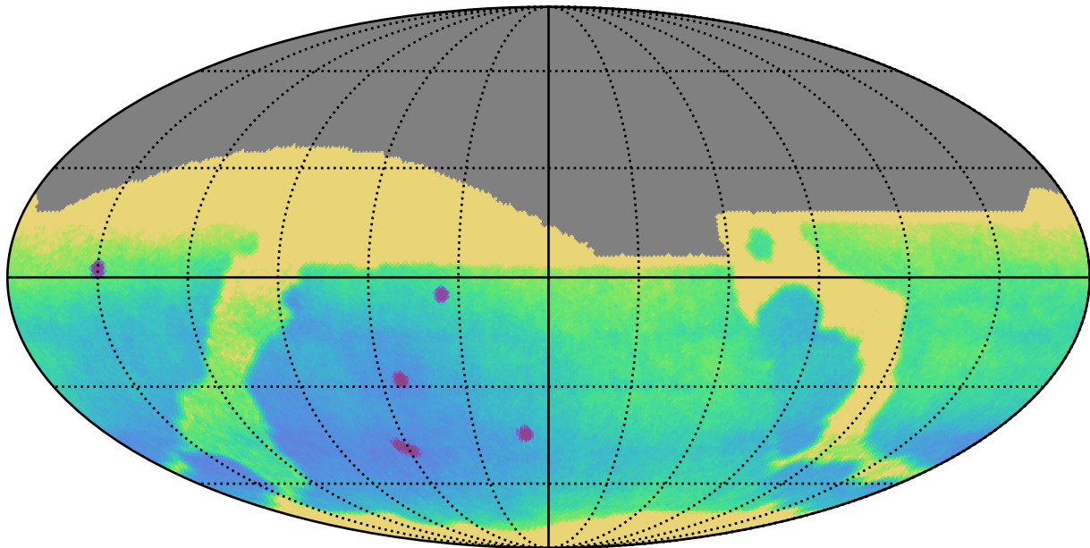
ddf_acor_sf20_lsf30_lsr10_v3.4_10yrs : Parallax Uncert @ 24.0
