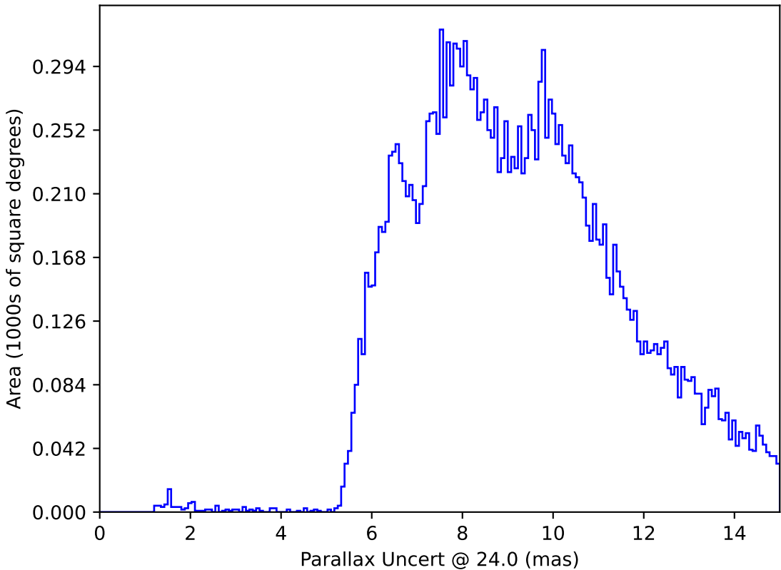
ddf_acor_sf20_lsf30_lsr10_v3.4_10yrs : Parallax Uncert @ 24.0
