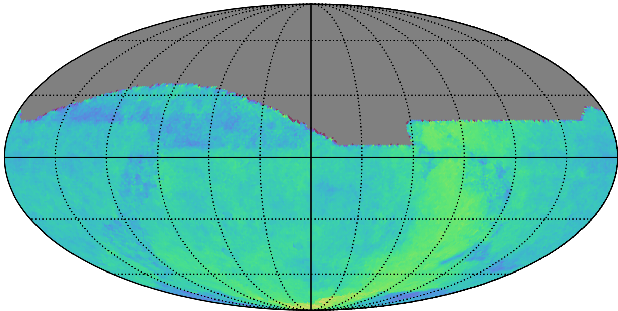
ddf_acor_sf20_lsf30_lsr10_v3.4_10yrs : Parallax Coverage @ 24.0
