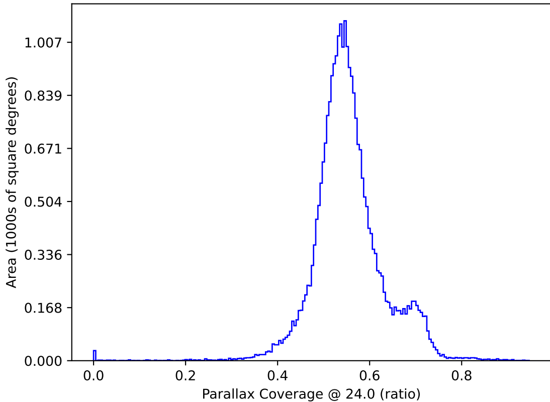
ddf_acor_sf20_lsf30_lsr10_v3.4_10yrs : Parallax Coverage @ 24.0
