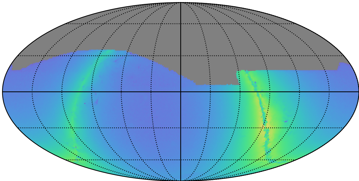
ddf_acor_sf20_lsf30_lsr10_v3.4_10yrs r: Nstars_no_crowding
