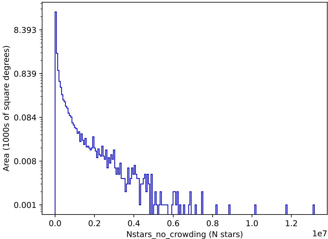
ddf_acor_sf20_lsf30_lsr10_v3.4_10yrs g: Nstars_no_crowding
