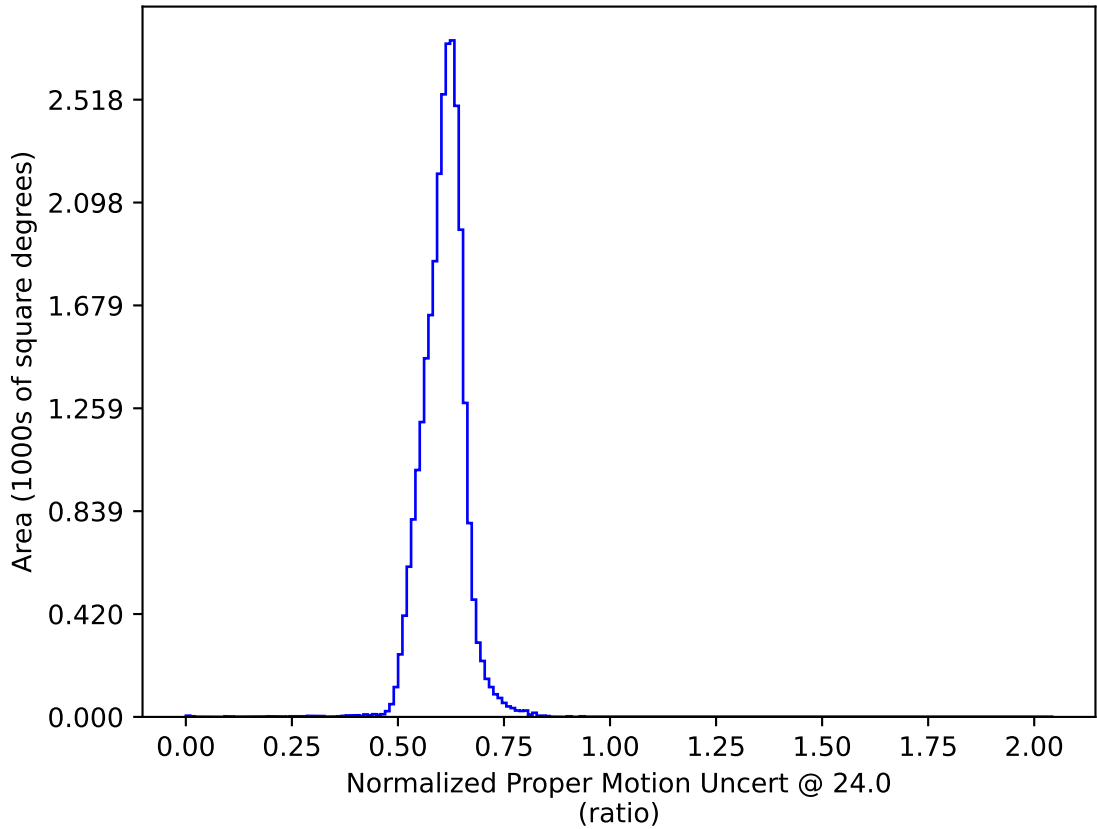
ddf_acor_sf20_lsf30_lsr10_v3.4_10yrs : Normalized Proper Motion Uncert @ 24.0
