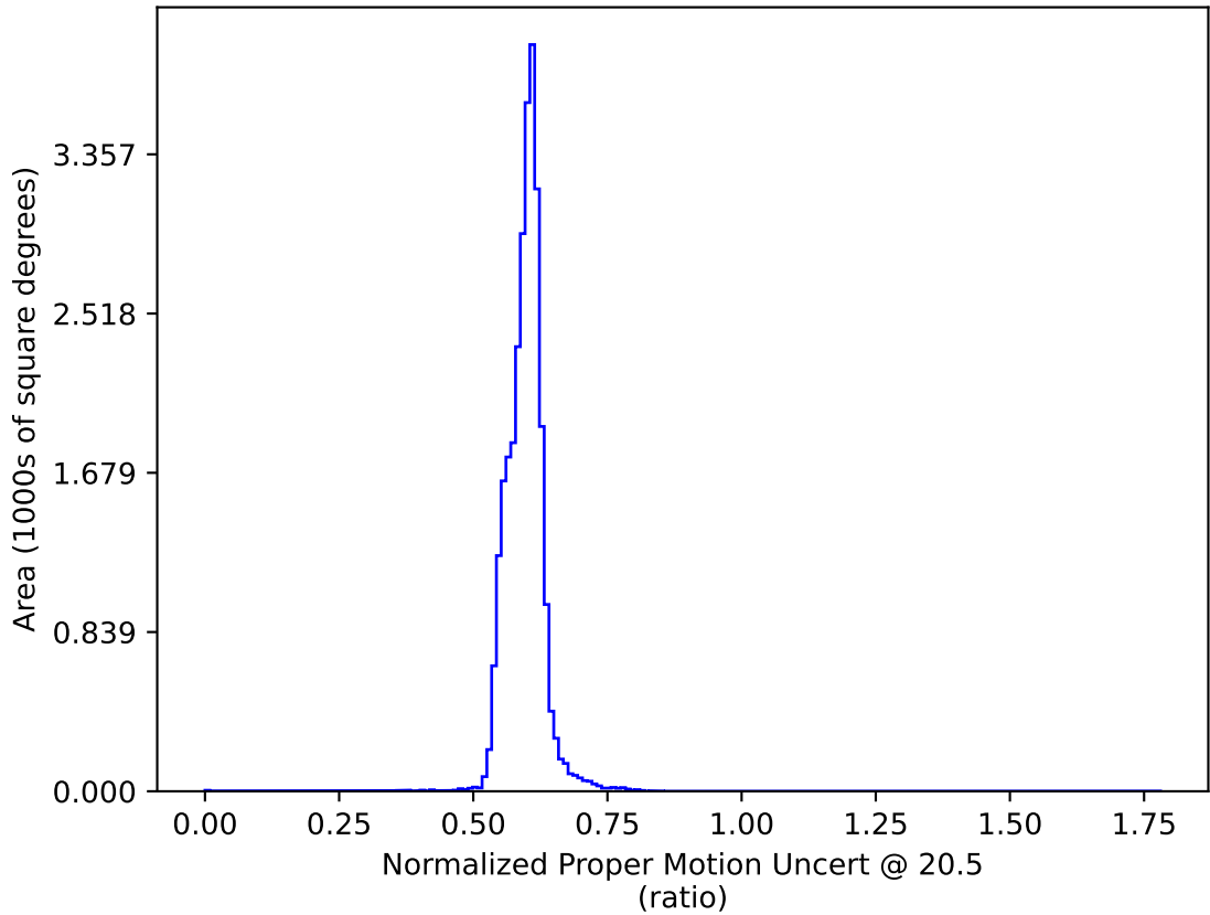
ddf_acor_sf20_lsf30_lsr10_v3.4_10yrs : Normalized Proper Motion Uncert @ 20.5
