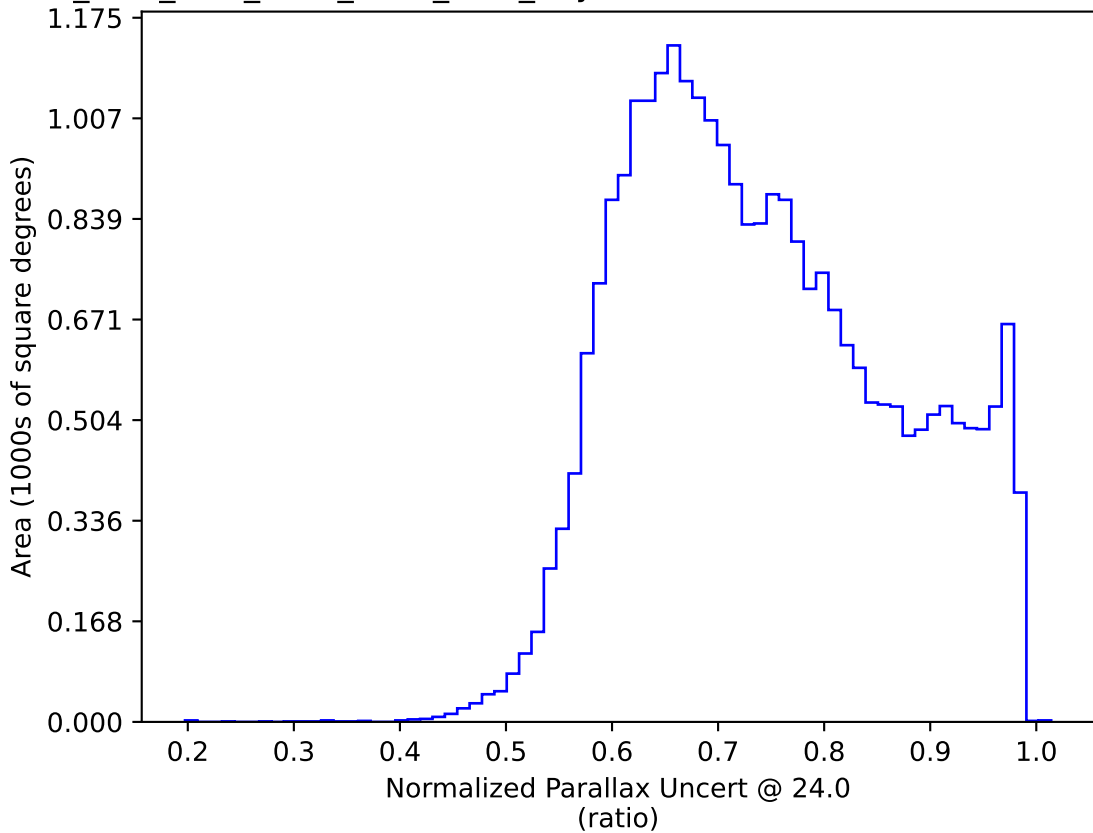
ddf_acor_sf20_lsf30_lsr10_v3.4_10yrs : Normalized Parallax Uncert @ 24.0
