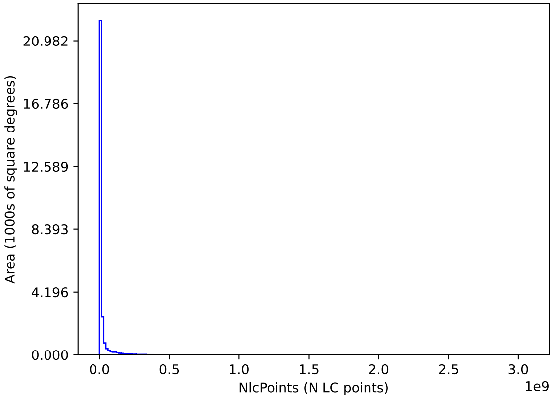
ddf_acor_sf20_lsf30_lsr10_v3.4_10yrs : NlcPoints
