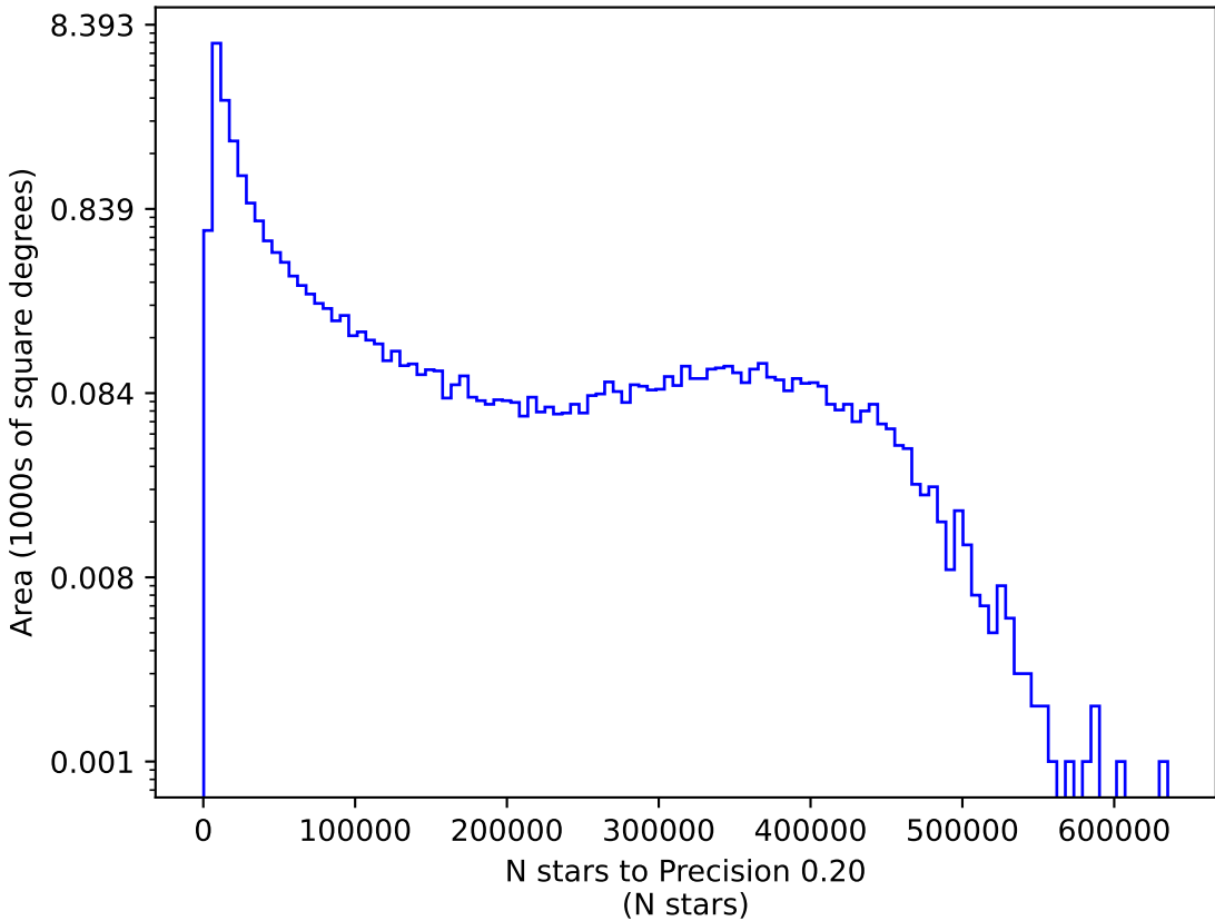
ddf_acor_sf20_lsf30_lsr10_v3.4_10yrs y: N stars to Precision 0.20
