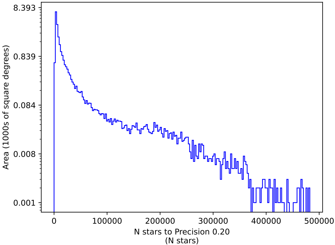
ddf_acor_sf20_lsf30_lsr10_v3.4_10yrs u: N stars to Precision 0.20
