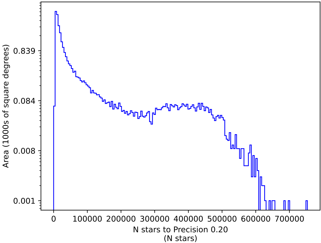
ddf_acor_sf20_lsf30_lsr10_v3.4_10yrs r: N stars to Precision 0.20
