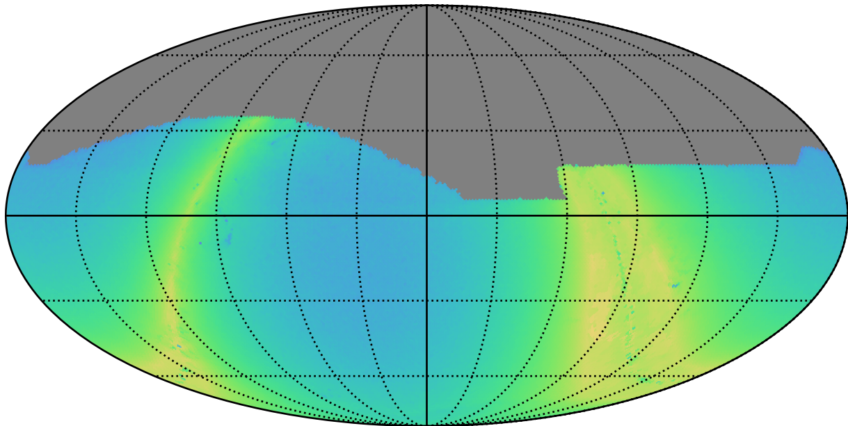
ddf_acor_sf20_lsf30_lsr10_v3.4_10yrs i: N stars to Precision 0.20
