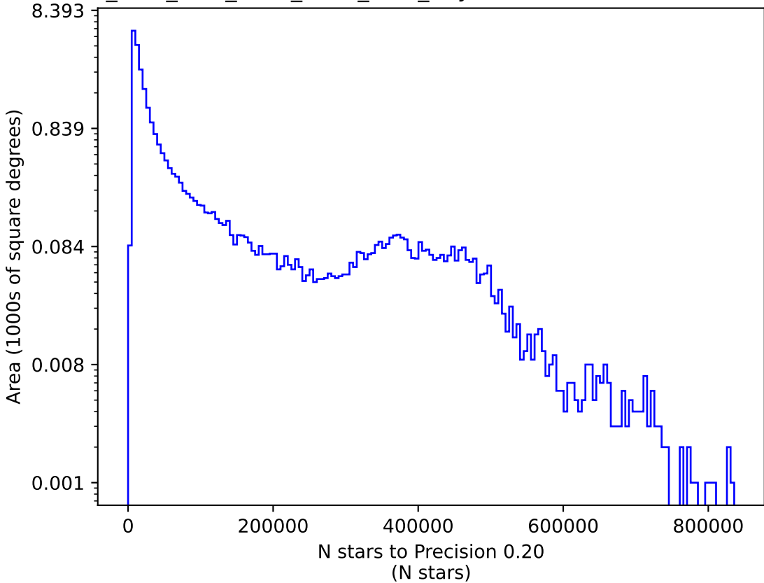
ddf_acor_sf20_lsf30_lsr10_v3.4_10yrs i: N stars to Precision 0.20
