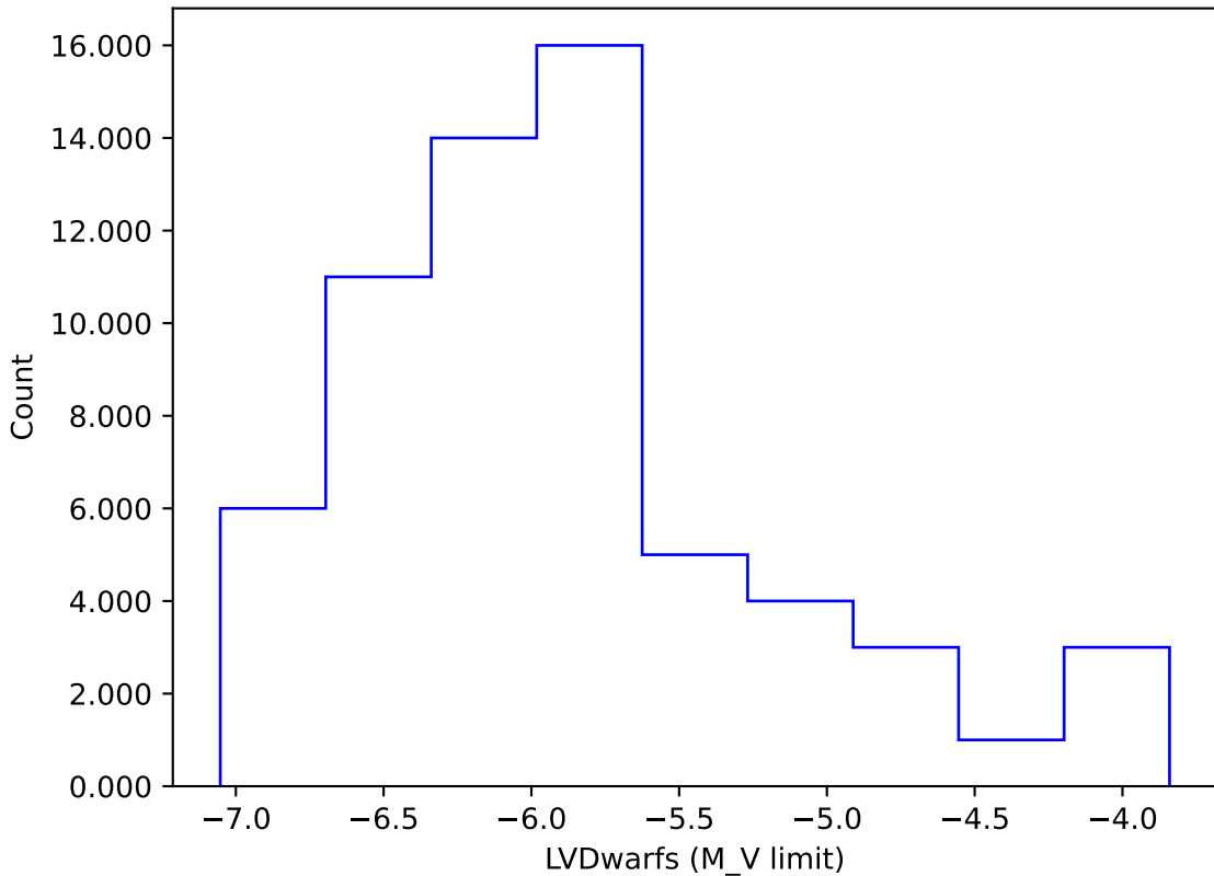
ddf_acor_sf20_lsf30_lsr10_v3.4_10yrs gi: LVDwarfs
