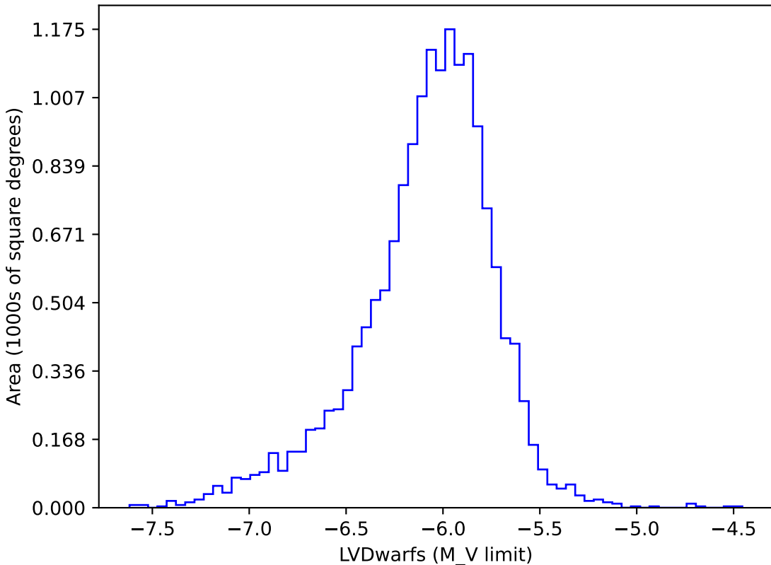
ddf_acor_sf20_lsf30_lsr10_v3.4_10yrs gi: LVDwarfs
