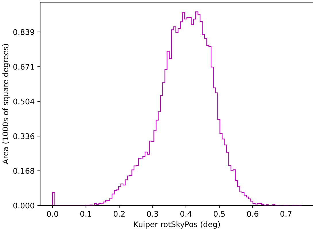
ddf_acor_sf20_lsf30_lsr10_v3.4_10yrs z: Kuiper rotSkyPos
