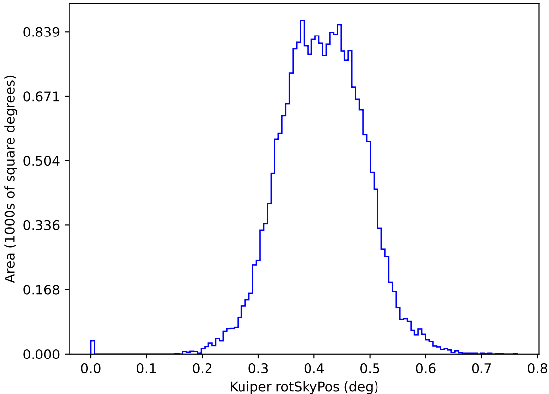
ddf_acor_sf20_ls30_lsr10_v3.4_10yrs y: Kuiper rotSkyPos
