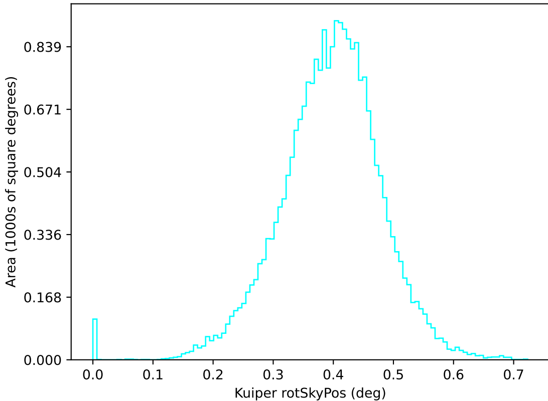
ddf_acor_sf20_lsf30_lsr10_v3.4_10yrs u: Kuiper rotSkyPos
