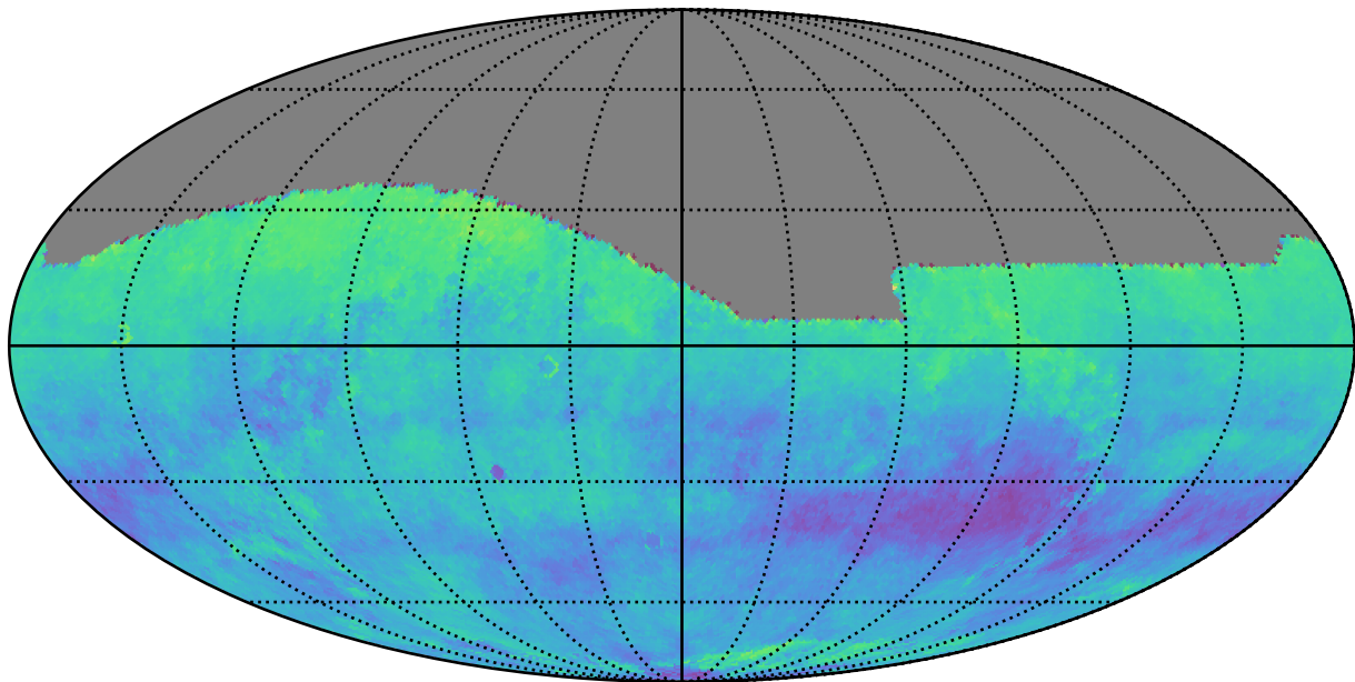
ddf_acor_sf20_lsf30_lsr10_v3.4_10yrs r: Kuiper rotSkyPos
