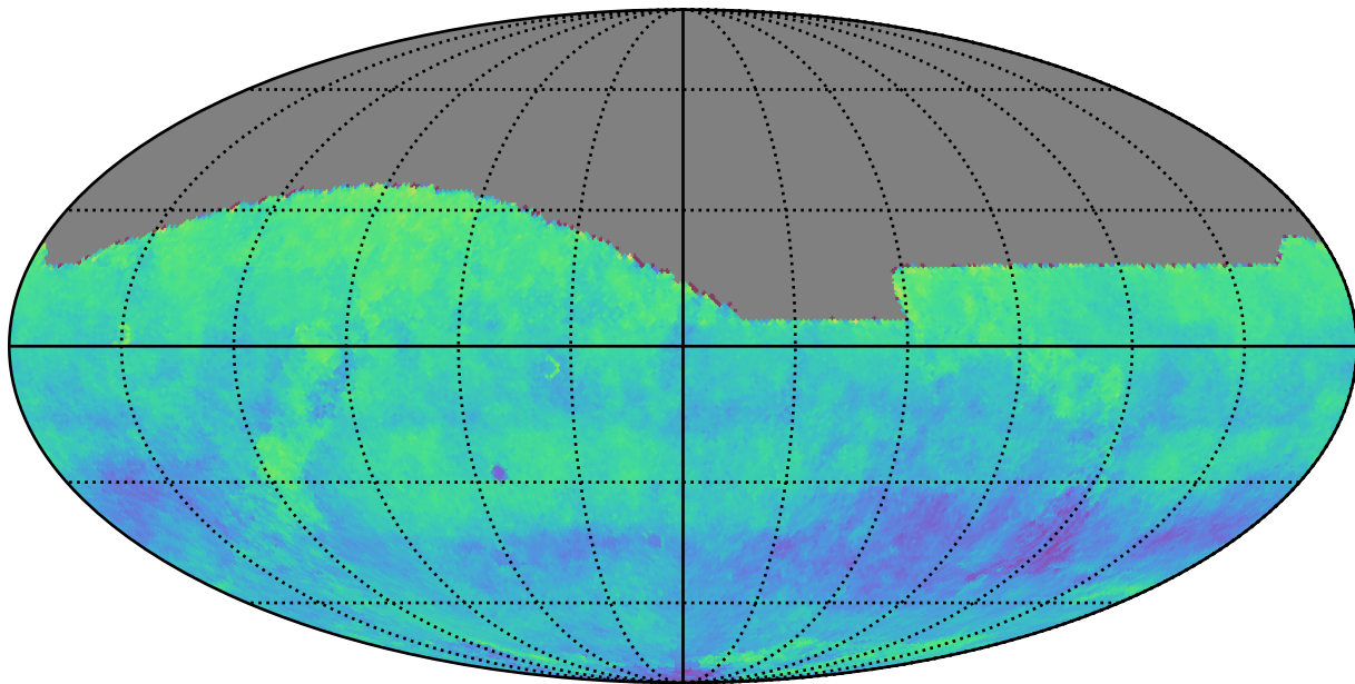
ddf_acor_sf20_lsf30_lsr10_v3.4_10yrs i: Kuiper rotSkyPos
