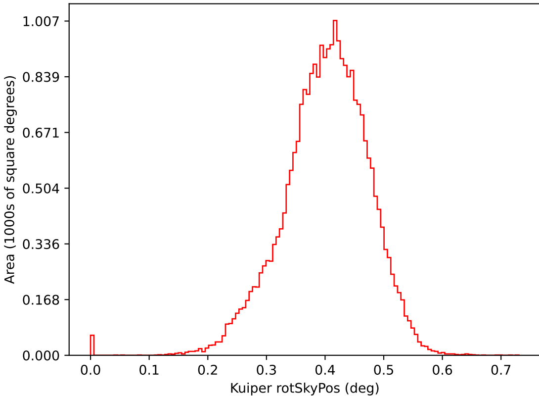
ddf_acor_sf20_lsf30_lsr10_v3.4_10yrs i: Kuiper rotSkyPos
