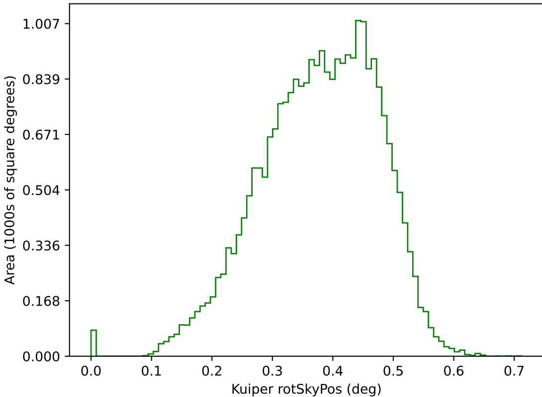
ddf_acor_sf20_lsf30_lsr10_v3.4_10yrs g: Kuiper rotSkyPos
