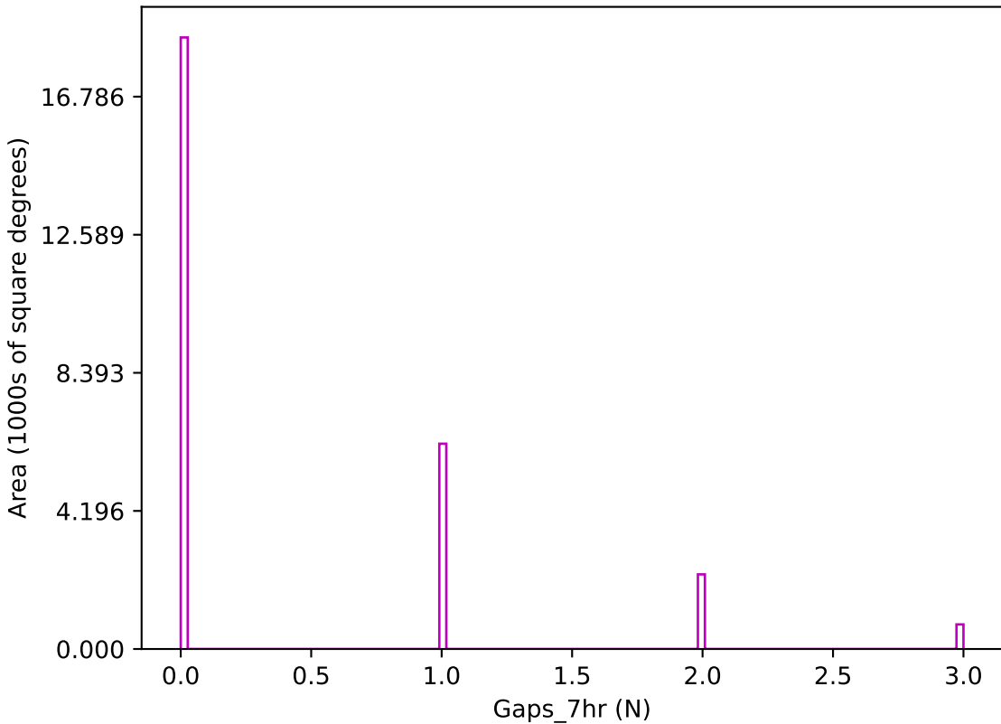
ddf_acor_sf20_ls30_lsr10_v3.4_10yrs z band: Gaps_7hr
