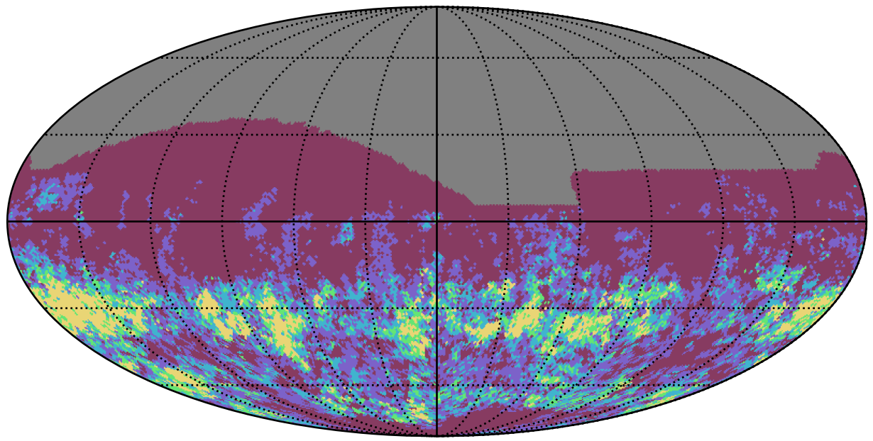
ddf_acor_sf20_lsf30_lsr10_v3.4_10yrs r band: Gaps_7hr
