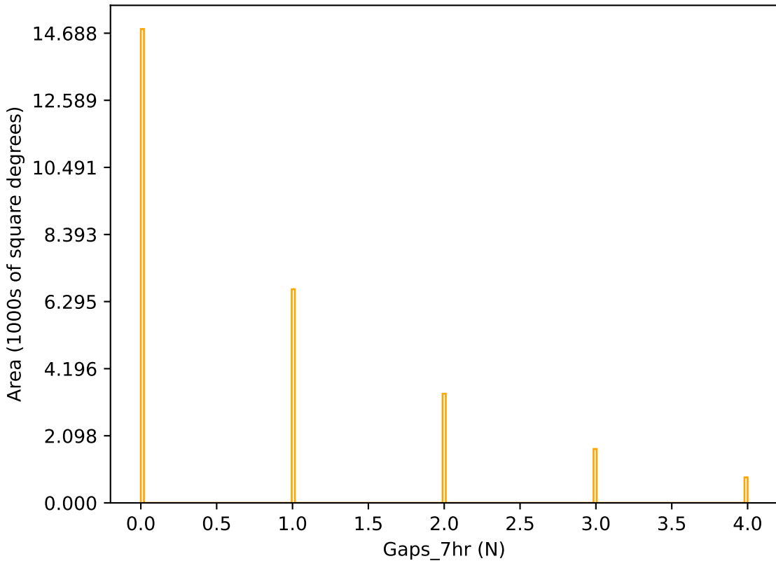
ddf_acor_sf20_lsf30_lsr10_v3.4_10yrs r band: Gaps_7hr
