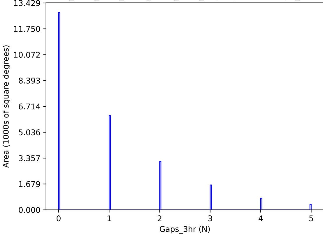
ddf_acor_sf20_lsf30_lsr10_v3.4_10yrs y band: Gaps_3hr
