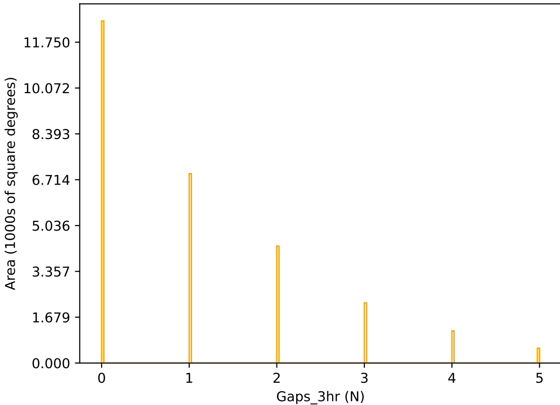
ddf_acor_sf20_lsf30_lsr10_v3.4_10yrs r band: Gaps_3hr
