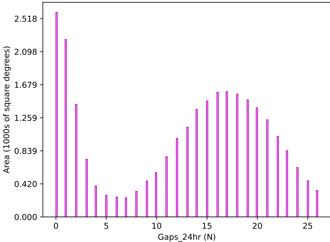
ddf_acor_sf20_lsf30_lsr10_v3.4_10yrs z band: Gaps_24hr
